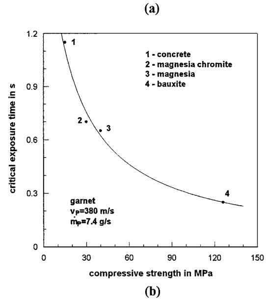
Figure 11 Relationship between local exposure time and erosion rate: (a) Target material influence and (b) Compressive strength and critical local exposure time.
