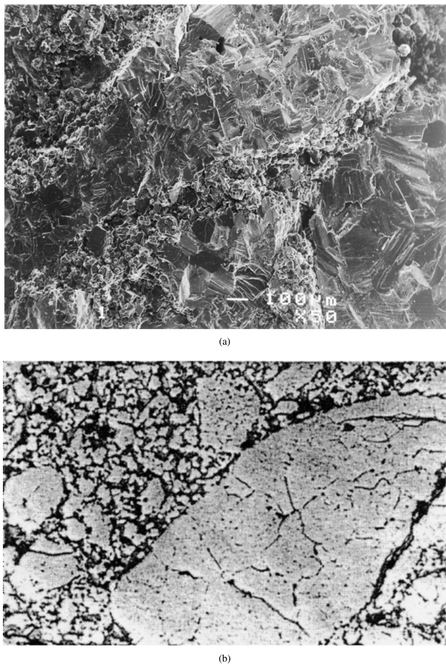
Figure 6 Structure and behaviour of sintered magnesia: (a) Brittle fracture under mechanical load and (b) Basic structure.
