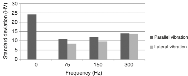
Fig. 15. Standard deviation of hardness distribution from the bottom of the buildup to 3 mm of its height.
