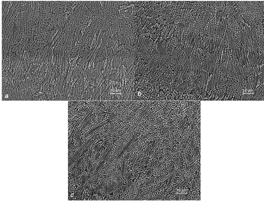
Fig. 11. Micrographs of the columnar dendrite at zone A under lateral vibration. (a) Vibration frequency: 75 Hz. (b) Vibration frequency: 150 Hz. (c) Vibration frequency: 300 Hz.
