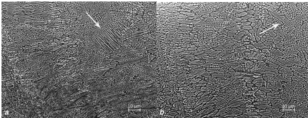
Fig. 12. Randomly-oriented grains showed by arrows, (a) 75 Hz lateral, (b) 150 Hz lateral.
