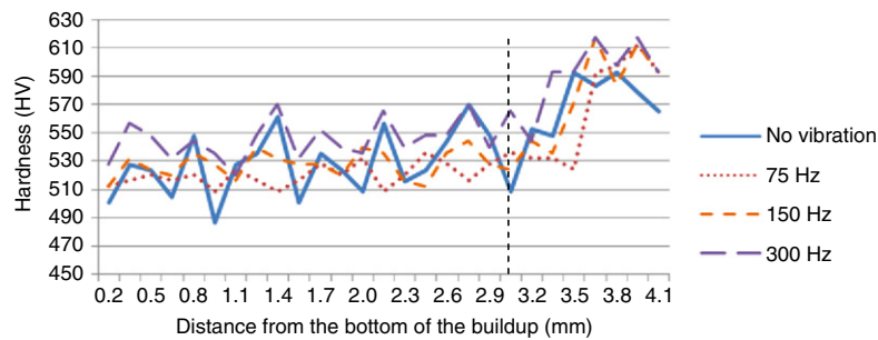
Fig. 14. Micro-hardness test results from the bottom to the top of the buildup for lateral vibration.
