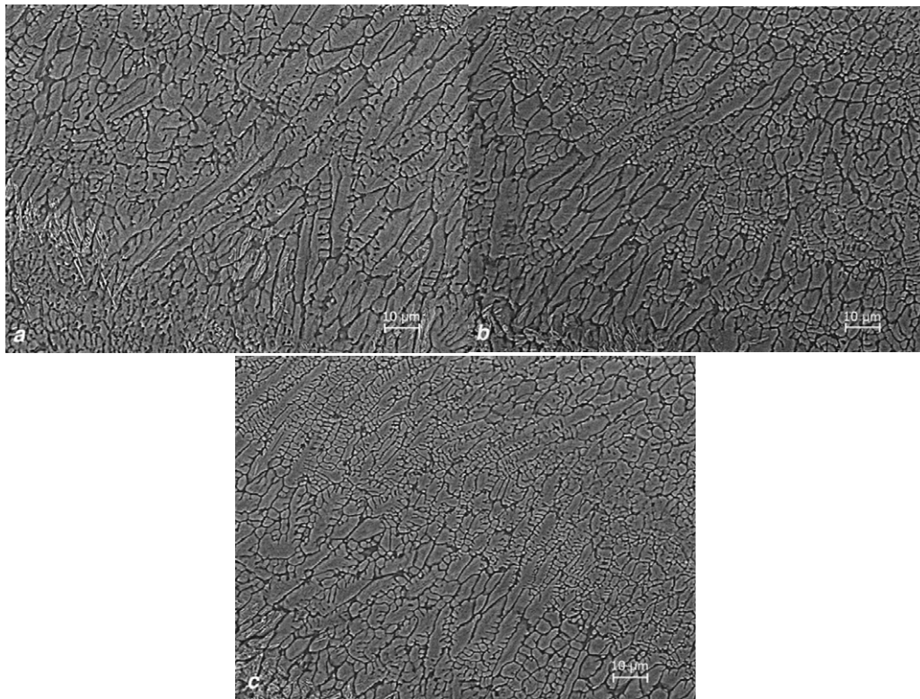
Fig. 10. Micrographs of the columnar dendrite at zone A under parallel vibration. (a) Vibration frequency: 75 Hz. (b) Vibration frequency: 150 Hz. (c) Vibration frequency: 300 Hz.
