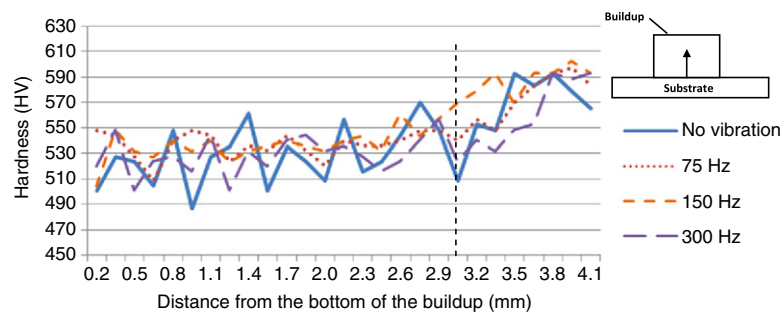
Fig. 13. Micro-hardness test results from the bottom to the top of the buildup for parallel vibration.
