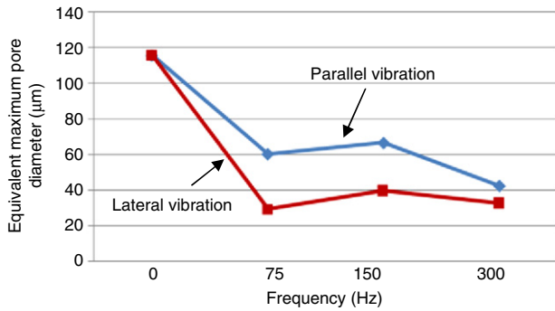
Fig. 8. Effect of vibration frequency and direction on equivalent maximum pore diameter.
